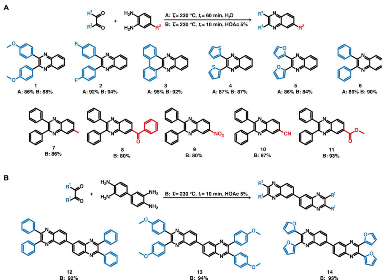
Scheme 2. Scope of 1,2-diketone and o -PDA in HTS of (A) quinoxalines and (B) biquinoxalines ( p_r=20\text{--}22\text{ bar} ).
