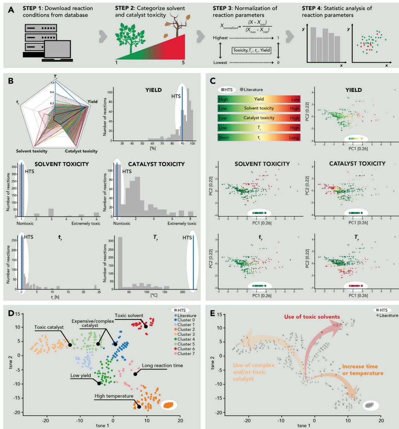
Figure 1. (A) Overview of the reaction parameter extraction pipeline. (B) Differences between HTS of quinoxalines and the reported literature synthesis. The spider plot depicts with dashed borders n=323 reactions that report all of the five parameters (solvent, catalyst, T_r , t_r and yield) used in the analysis. The black solid line indicates the average of all the 323 considered reactions whereas the blue solid line represents the average of HT conditions. Spider plots for individual compounds are included in the Supporting Information (Figure S36). The different histograms were plotted considering the number of reactions that report the corresponding parameter: solvent ( n=452 ), catalyst ( n=484 ), T_r ( n=479 ), t_r ( n=538 ), yield ( n=513 ). (C) Reaction space of 2,3-diarylquinoxalines with overlay of the 5 investigated features. Green depicts a more favourable reaction parameter whereas red indicates less favourable conditions. (D) t-SNE dimension reduction depicting clusters of favourable reaction conditions. (E) Possible reaction strategies to improve reaction yields.
