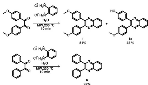
Scheme 4. Reaction between o -PDA dihydrochloride and 1,2-diketones under HT conditions ( p_r=20\text{--}22\text{ bar} ).
