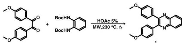
Scheme 3. One-pot Boc-deprotection-quinoxaline formation sequence under HT conditions ( p_r=20\text{--}22\text{ bar} ). Yields: 73 % with t_r=10\text{ min} and 76 % with t_r=30\text{ min} .
